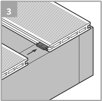
Install hidden fasteners to fit the next board in place.
