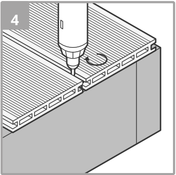
Tighten hidden fastener screws to secure the boards.
