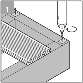
Fix starter clips to the outer edge of your deck.
