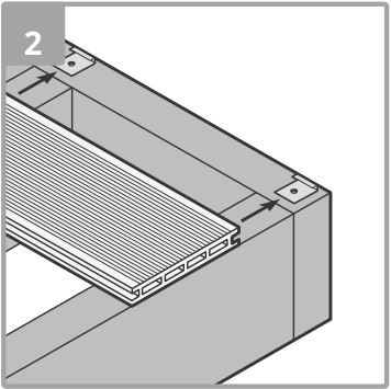
Slide the first board into the starter fastener.
